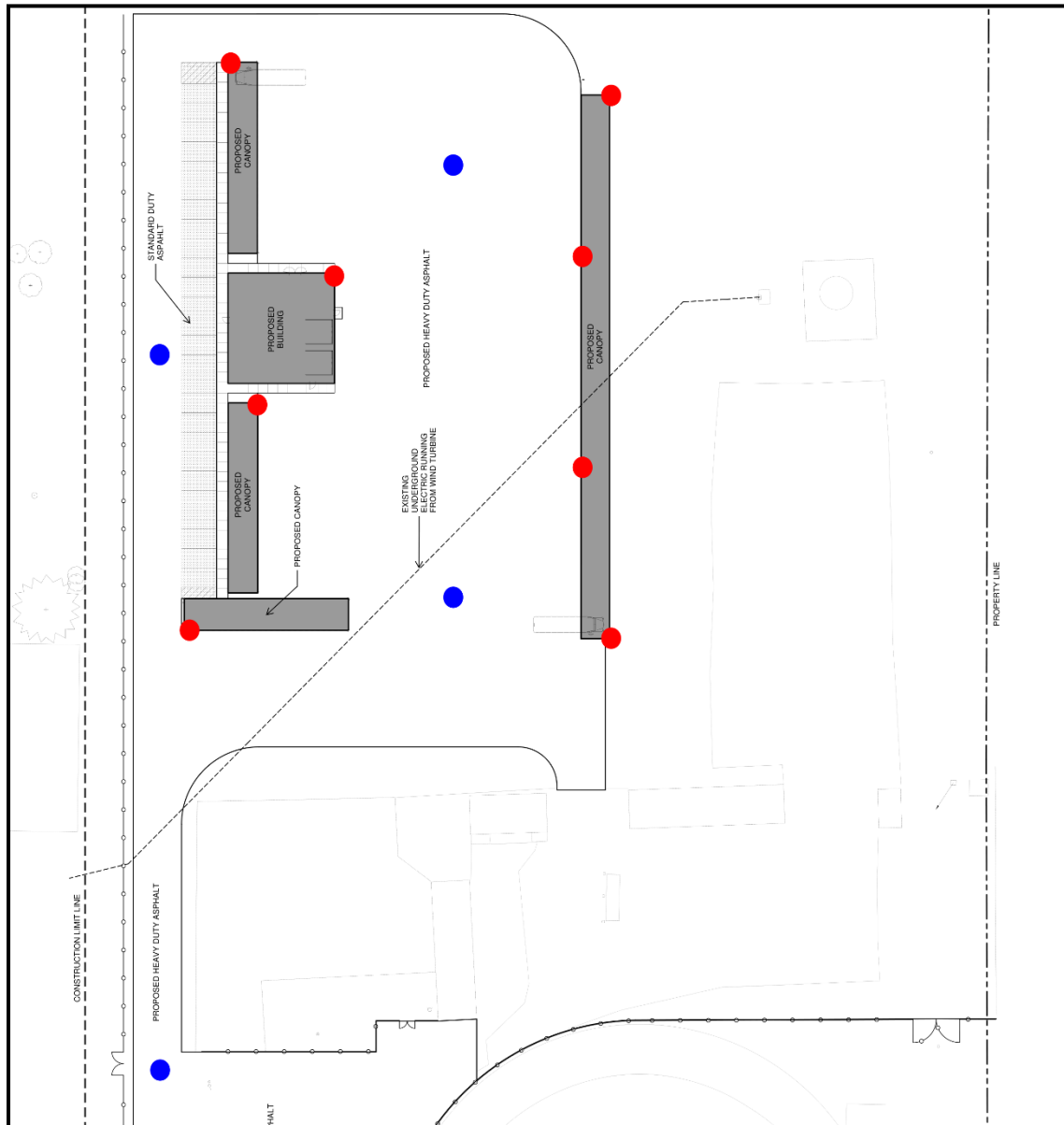
Figure 1 – Conceptual/Preliminary Plan (dated March 12, 2026) of Planned Construction
